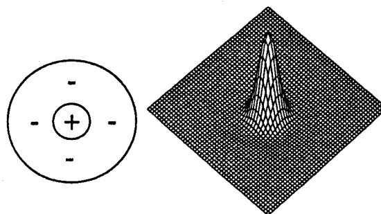
Fig. 1. Receptive fields, input filtering. a) Conventional representation of a circularly symmetric receptive field (e.g., of a retinal ganglion cell). b) 3D representation of (a) as the impulse function of a filter.
